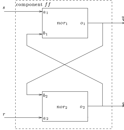
Figure 7.2: RS-flip-flop example
