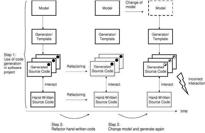
Fig. 1. Risk of incompatibility when refactoring generated source code.
